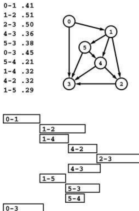
Figure 21.25 A PERT chart
