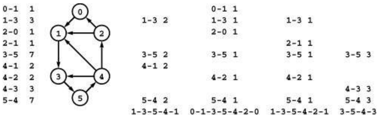
Figure 22.8 Cycle flow representation
