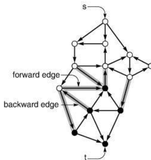
Figure 22.14 st -cut terminology
