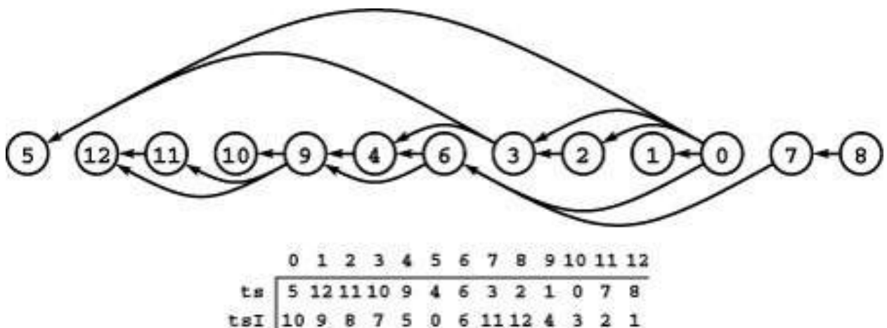
Figure 19.23 Reverse topological sort
