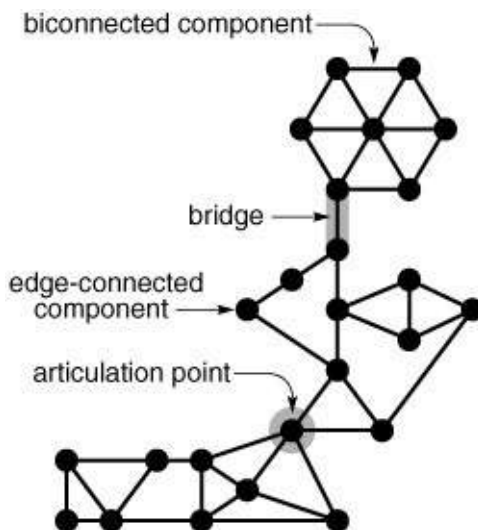
Figure 18.19 Graph separability terminology
