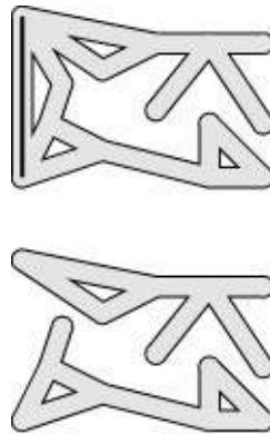
Figure 18.4 Decomposing a maze
