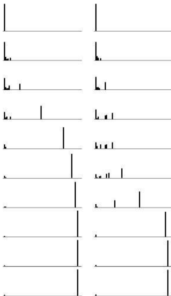
Figure 18.30 Connectivity in random graphs
