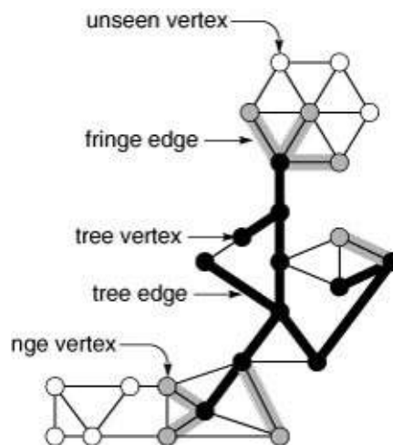
Figure 18.26 Graph search terminology
