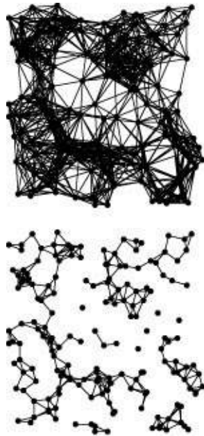
Figure 20.19 Euclidean near-neighbor graphs
