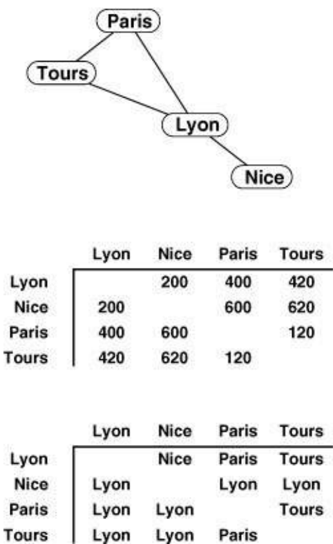
Figure 21.4 Distances and paths
