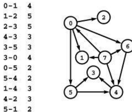
Figure 22.52 Mail carrier's problem
