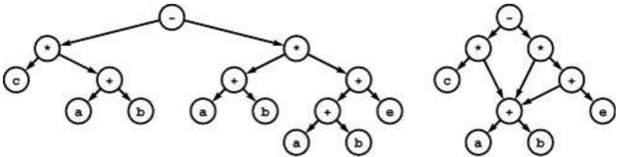
Figure 19.19 DAG representation of an arithmetic expression
