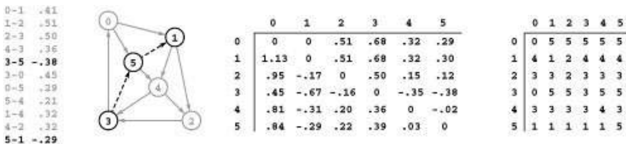
Figure 21.26 A sample network with negative edges
