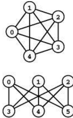
Figure 17.24 Forbidden subgraphs in planar graphs
