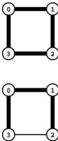
Figure 20.7 Cycles in Boruvka's algorithm
