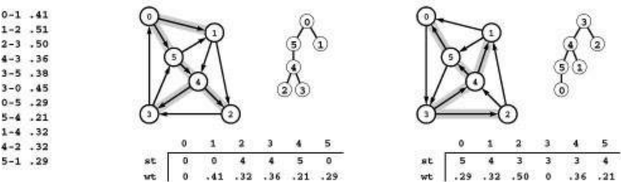
Figure 21.6 Shortest paths trees
