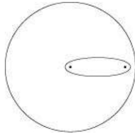
Figure 21.20 Euclidean heuristic cost bounds
