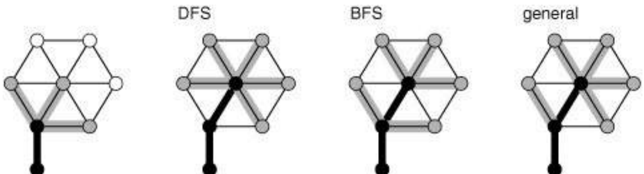
Figure 18.27 Graph search strategies
