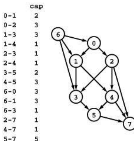
Figure 22.36 Reduction from feasible flow
