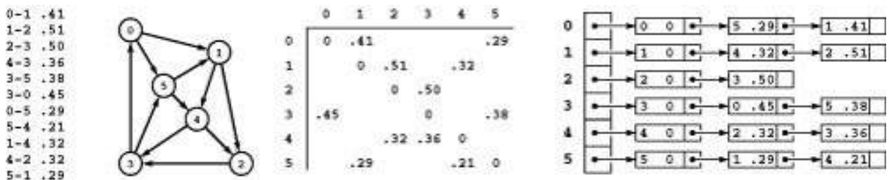
Figure 21.1 Sample network and representations
