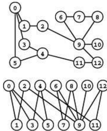
Figure 17.5 A bipartite graph
