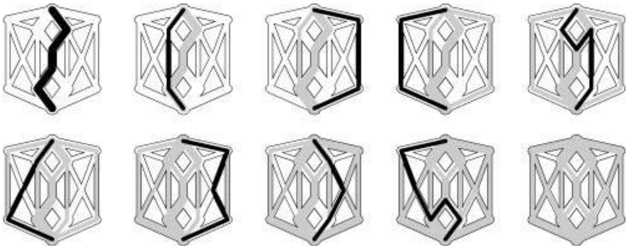
Figure 22.18 Maximum-capacity augmenting paths
