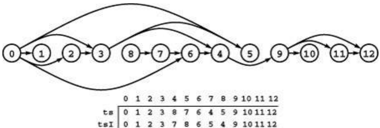
Figure 19.22 Topological sorting (rearrangement)
