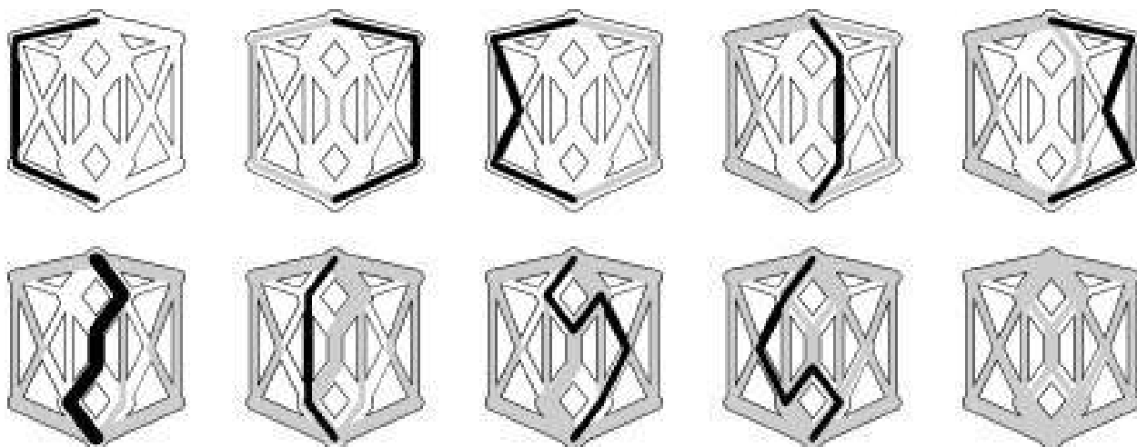
Figure 22.21 Randomized augmenting-path search
