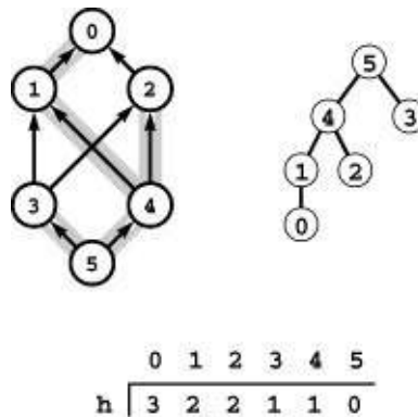
Figure 22.27 Initial height function
