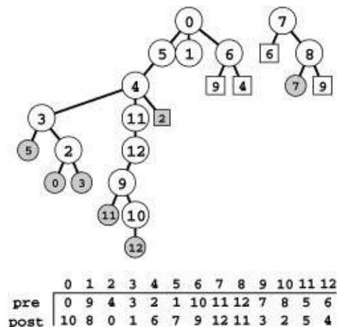
Figure 19.9 DFS forest for a digraph
