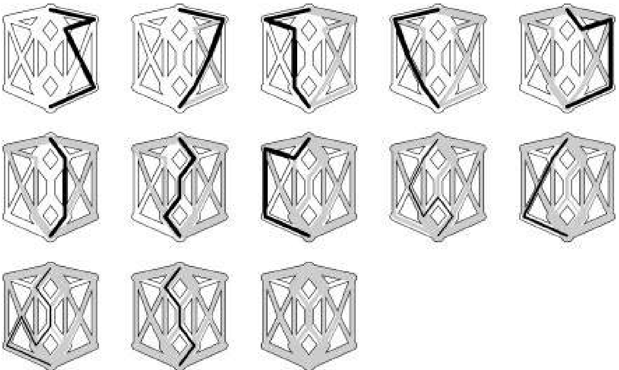
Figure 22.20 Stack-based augmenting-path search
