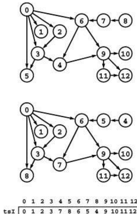
Figure 19.21 Topological sort (relabeling)
