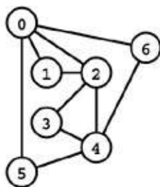
Figure 17.17 Trace for simple path search
