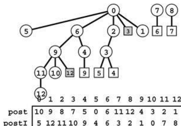
Figure 19.24 DFS forest for a DAG
