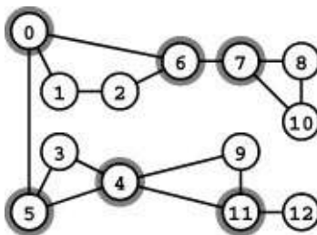
Figure 18.20 Articulation points (separation vertices)
