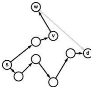
Figure 21.18 Edge relaxation (Euclidean)
