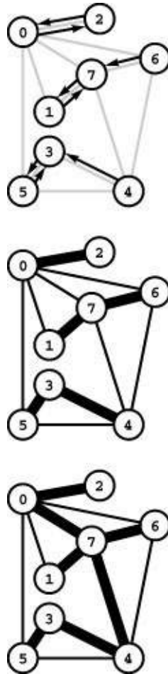
Figure 20.14 Boruvka's MST algorithm
