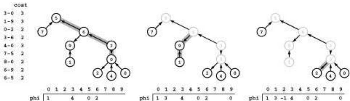
Figure 22.47 Computing potentials through parent links
