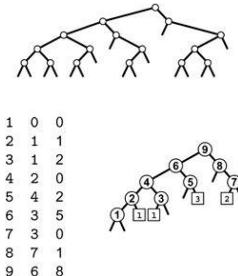
Figure 19.20 Binary tree compression
