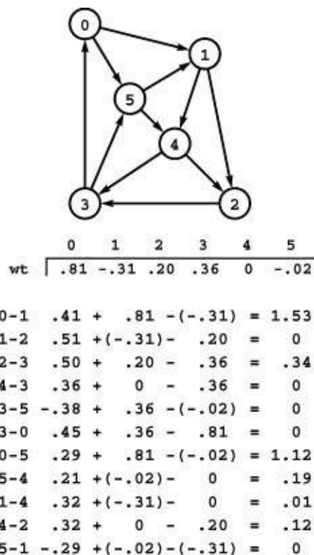
Figure 21.31 Reweighting a network
