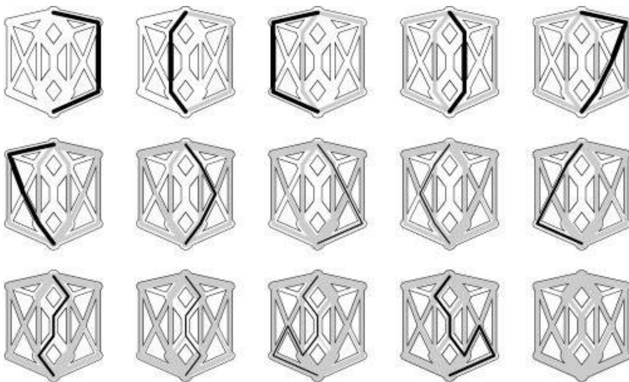
Figure 22.17 Shortest augmenting paths
