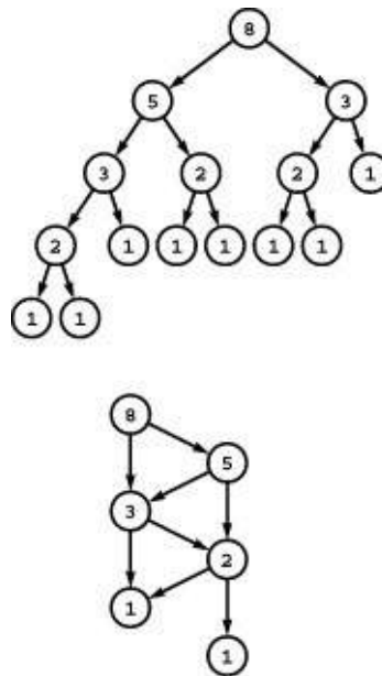
Figure 19.18 DAG model of Fibonacci computation
