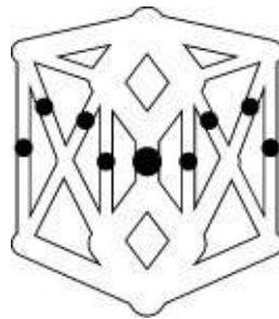
Figure 22.4 Cutting supply lines
