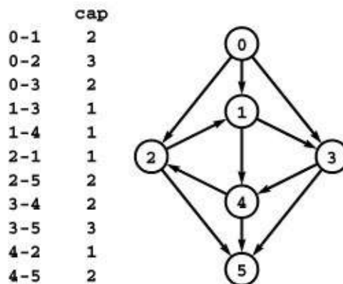
Figure 22.11 Flow network with cycle
