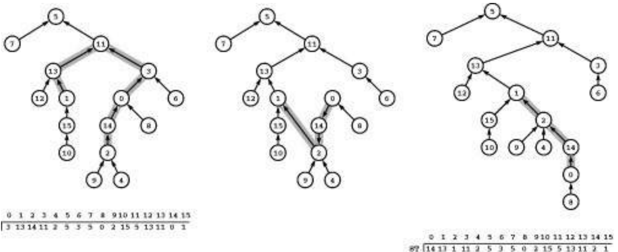
Figure 22.48 Spanning tree substitution
