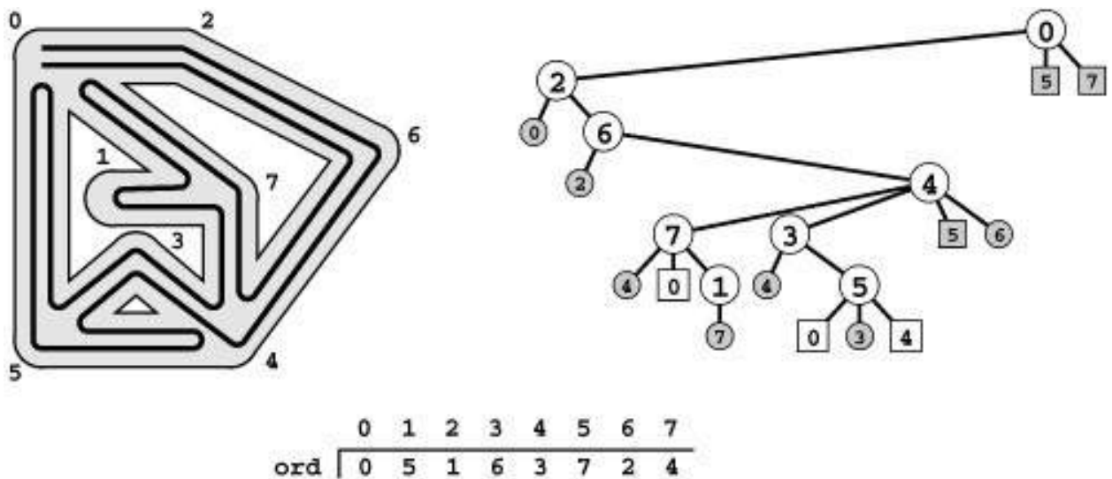
Figure 18.14 A two-way Euler tour
