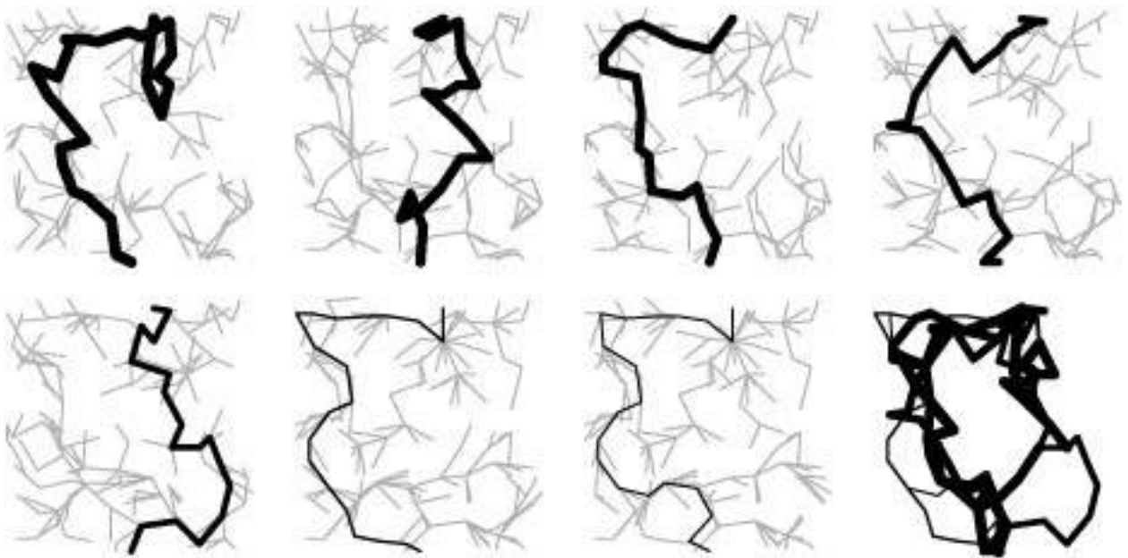
This figure depicts the augmenting paths computed by the maximum-capacity algorithm for the Euclidean network with random weights that is shown in Program 22.22, along with the edges in the graph-search spanning tree (in gray). The resulting flow is shown at the bottom right.
