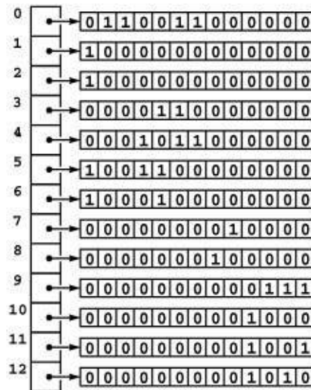
Figure 17.9 Adjacency matrix data structure
