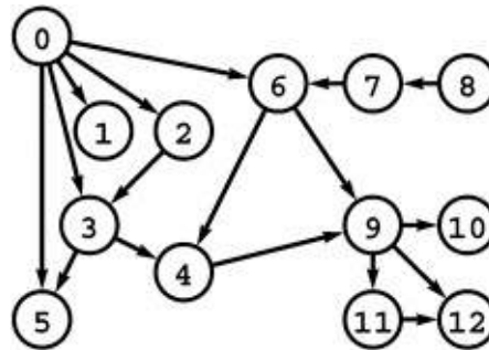
Figure 19.6 A directed acyclic graph (DAG)
