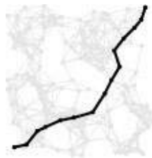
Figure 21.13 Diameter of a network
