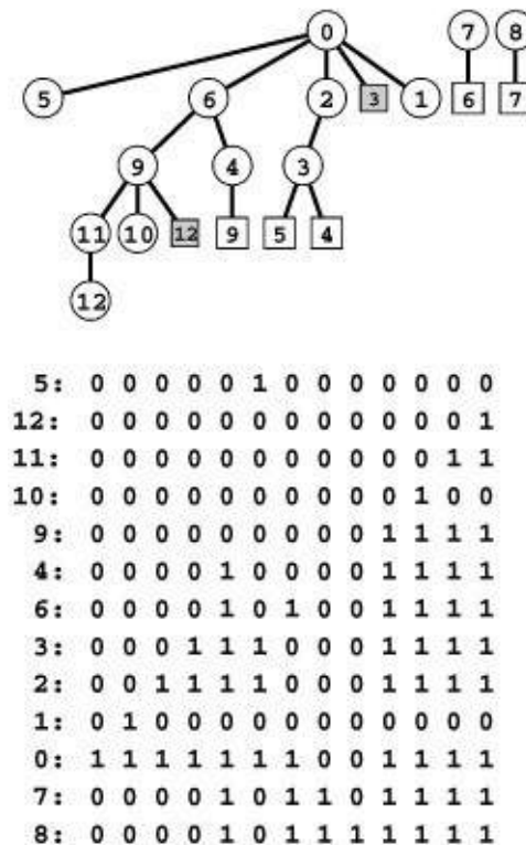
Figure 19.27 Transitive closure of a DAG
