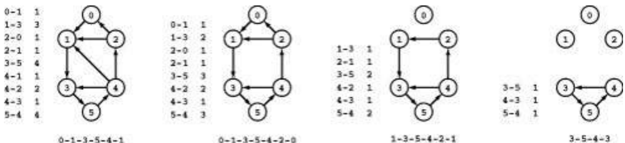
Figure 22.9 Cycle flow decomposition process
